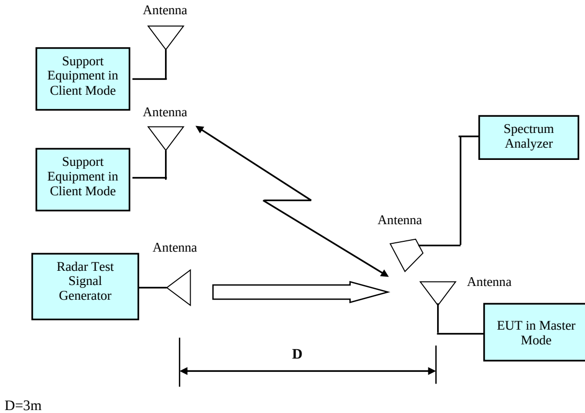
Setup for Radiated Method for Master Mode
