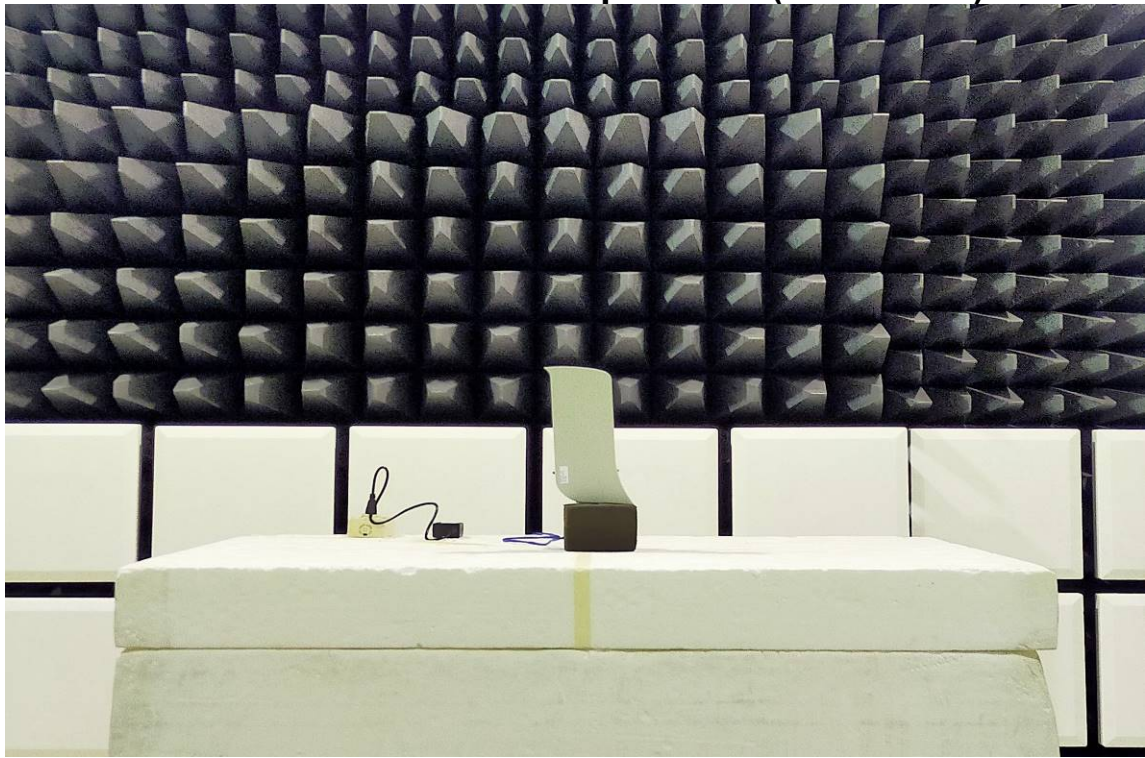
Radiated Emission Set up Photos (Front View)
