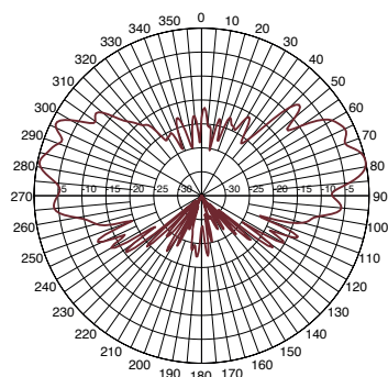
ELEVATION PATTERN
