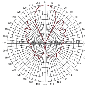
ELEVATION PATTERN
