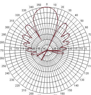
AZIMUTH PATTERN
