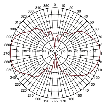
AZIMUTH PATTERN
