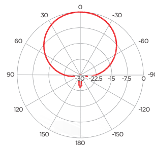
V/H - Port Pattern Azimuth 5.6 GHz
