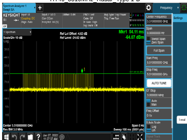
HT40_5510MHz_Radar_Type 1-B
