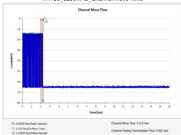
VHT80_5290MHz_Channel Move Time
