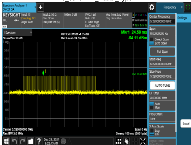
HT20_5320MHz_Radar_Type 1-B
