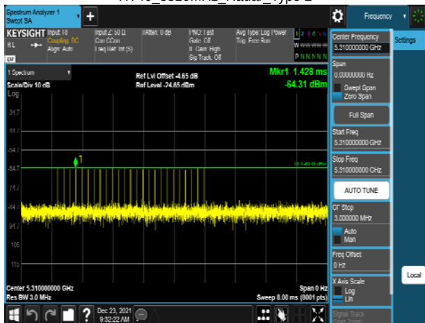
HT40_5310MHz_Radar_Type 3
