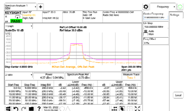
Emission Mask_Chain1_4980MHz
