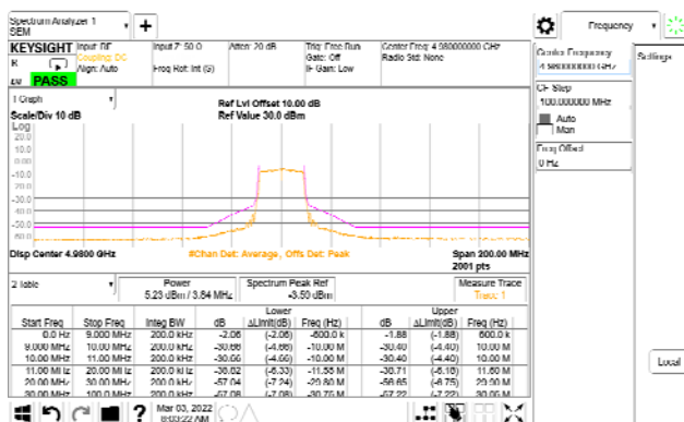
Emission Mask_Chain0_4980MHz
