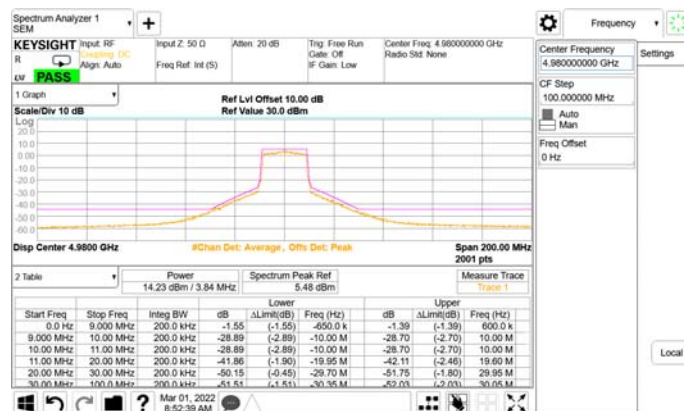
Emission Mask_Chain1_4980MHz
