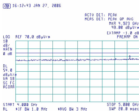
Plot 7.2.34 Radiated emission measurements at band edge at the high carrier frequency, bitrate 1 MBit/s
