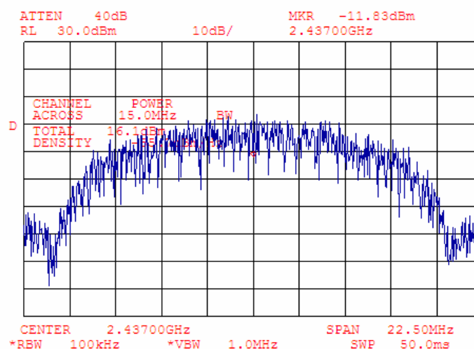
Plot 7.1.2 Peak output power at mid frequency
