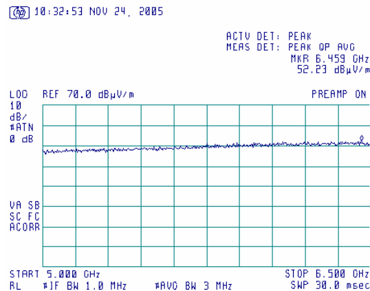
Plot 7.2.45 Radiated emission measurements from 5000 to 6500 MHz at the high carrier frequency
