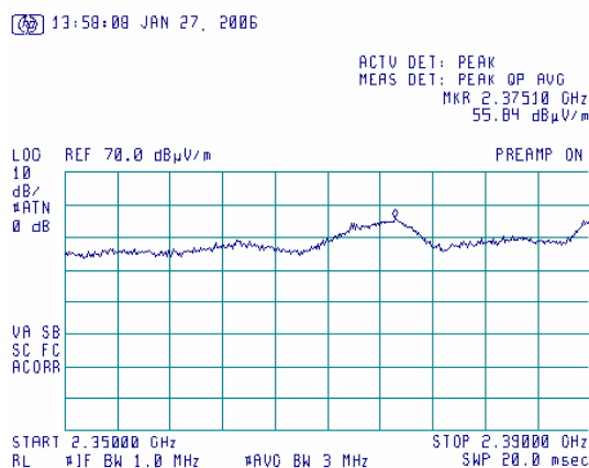
Plot 7.2.24 Radiated emission measurements at band edge at the low carrier frequency, bitrate 1 MBit/s
