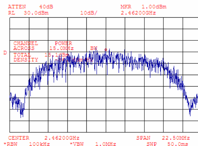
Plot 7.1.3 Peak output power at high frequency
