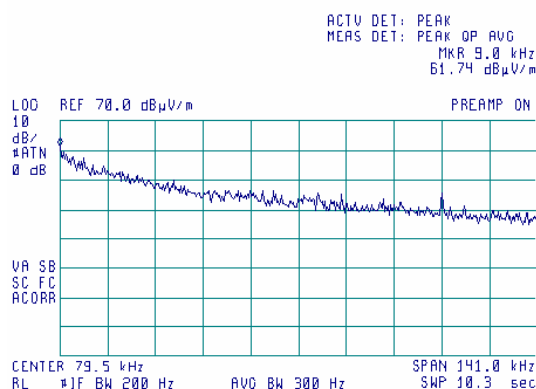
Plot 7.2.8 Radiated emission measurements from 9 to 150 kHz at the mid carrier frequency
