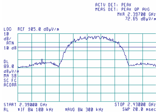
Plot 7.2.26 Radiated emission measurements at band edge at the low carrier frequency, bitrate 11 MBit/s
