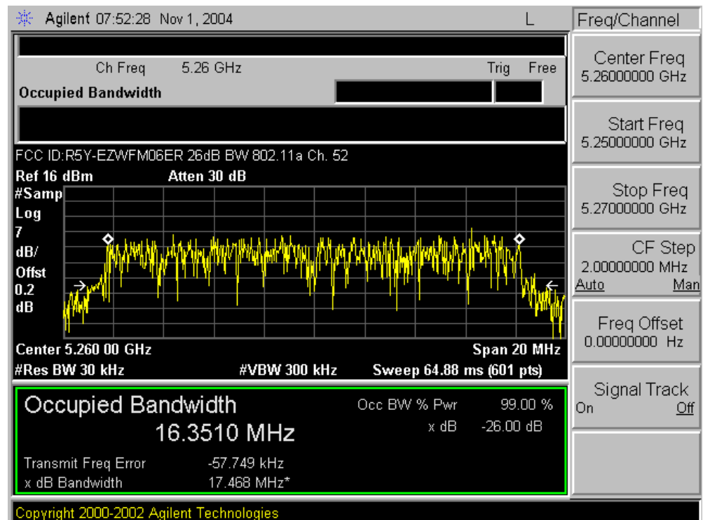
Plot A-2. 26dB Bandwidth Plot – Ch. 52
