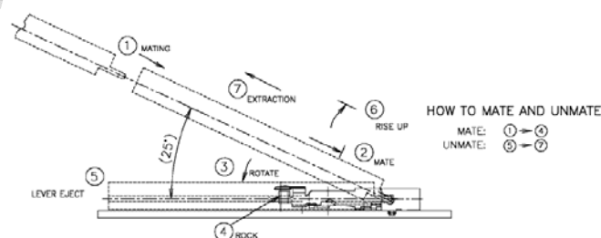
Figure 1.1: Insertion and Removal of the Mini-PCI Board
