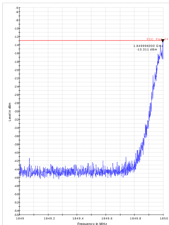
Diagram 37.10_BE_Ch512_GPRS_PK
