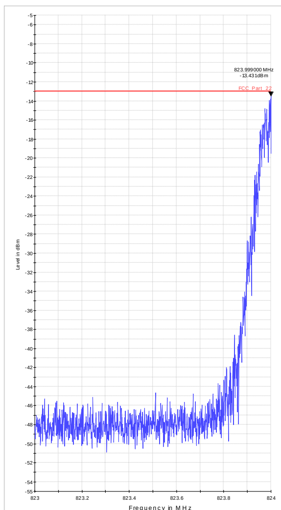
Diagram 37.03_BE_Ch128_GPRS
