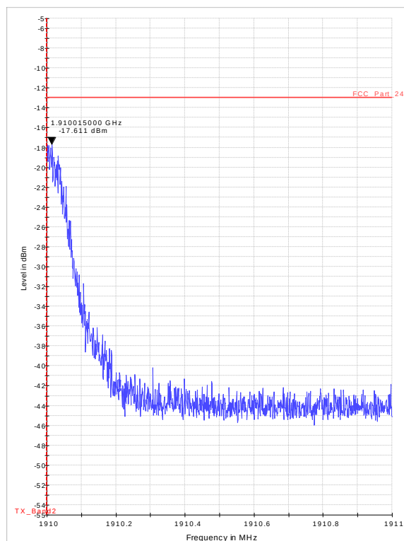
Diagram 37.13_BE_Ch810_EGPRS_PK
