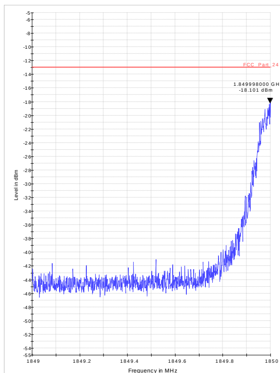
Diagram 37.12_BE_Ch512_EGPRS_PK
