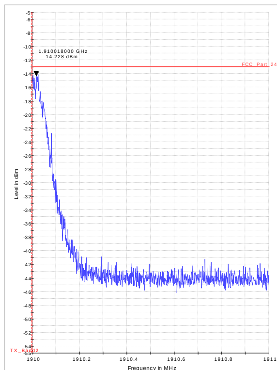
Diagram 37.11_BE_Ch810_GPRS_PK
