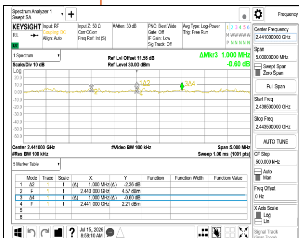
π/4DQPSK_2M_DH5_CH38CH39CH40
