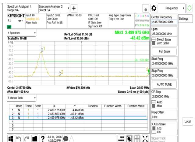
Band Edge_GFSK_1M_DH5_2480MHz
