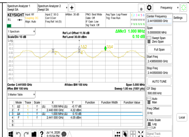
GFSK_1M_DH5_CH38CH39CH40
