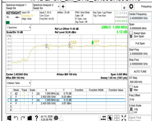
8DPSK_3M_DH5_CH0CH1CH2
