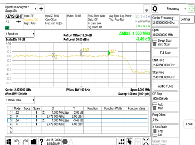
π/4DQPSK_2M_DH5_CH76CH77CH78
