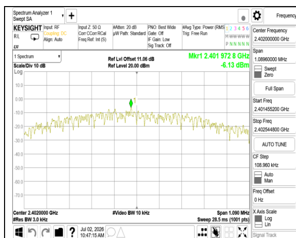
PSD_BLE_1M_2402MHz
