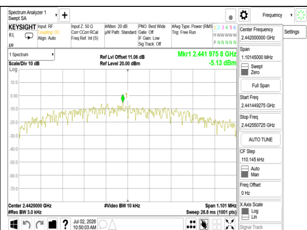
PSD_BLE_1M_2442MHz
