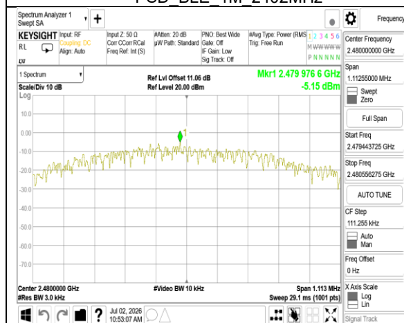
PSD_BLE_1M_2480MHz
