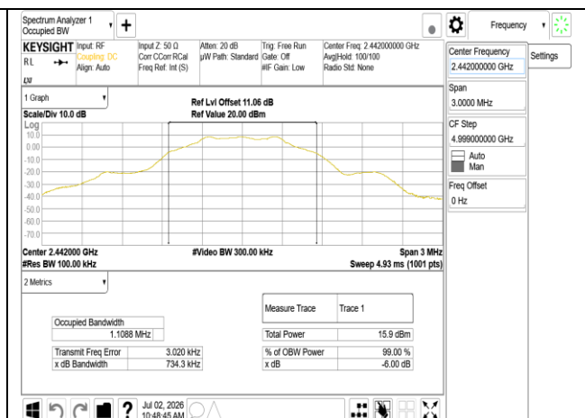
OBW 6dB_BLE_1M_2442MHz
