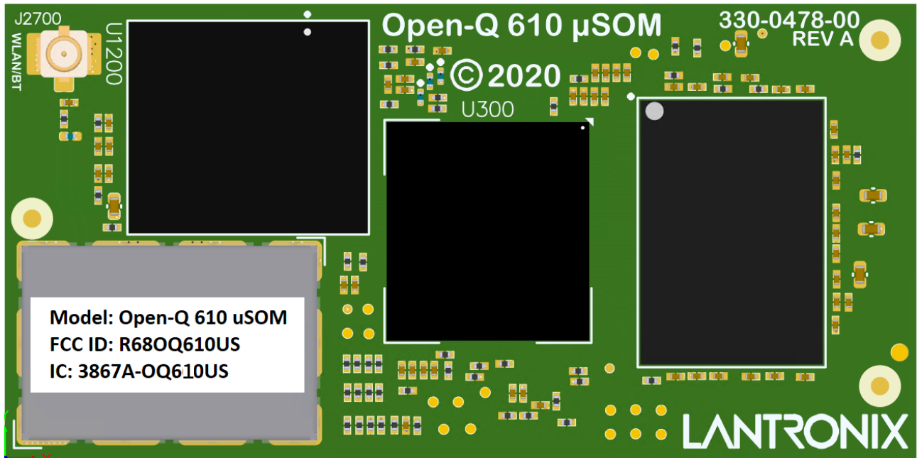
Top Side Drawing of Module with Label.
