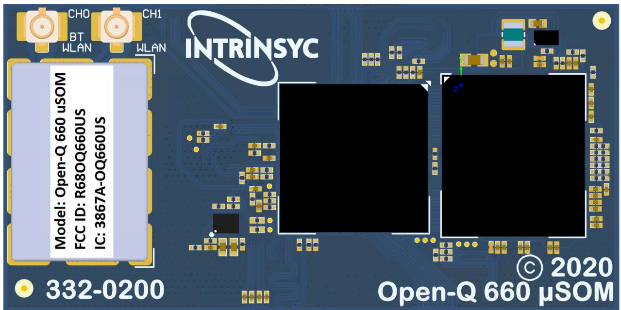
Top Side Drawing of Module with Label.
