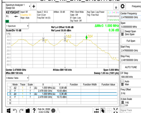
GFSK 1M_DH5_CH76CH77CH78
