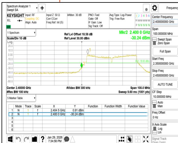
802.11n 40MHz Chain0 2422MHz
