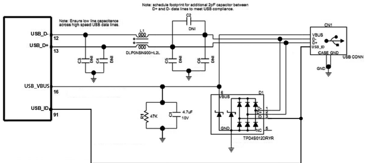
Figure 4-3: USB Interface
