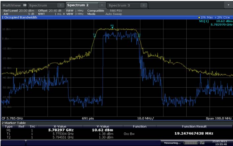
U-NII 3 Mid Channel 20MHz BW
