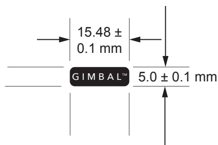
DEVICE EDGE BRANDING 100% SCALE
