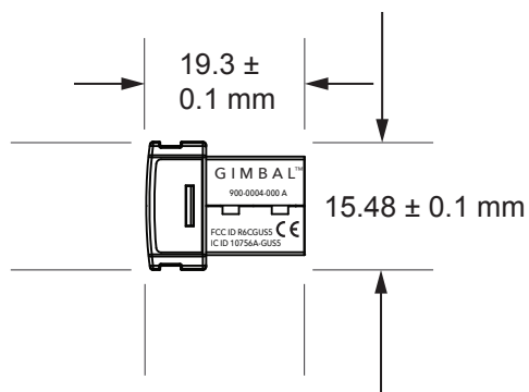
HOUSING ETCHING 100% SCALE
