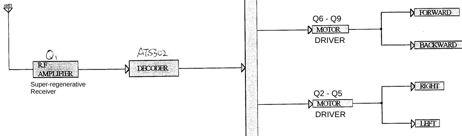
RX-40.680MHZ FUNCTION BLOCK DIAGRAM
