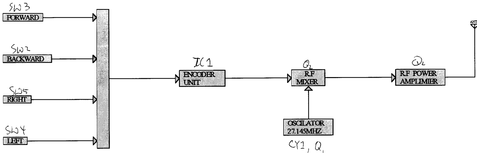
FUNCTION BLOCK DIAGRAM
