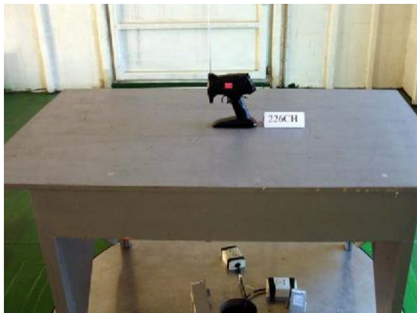
Photo 2: Radiated Emission Test Set-up
