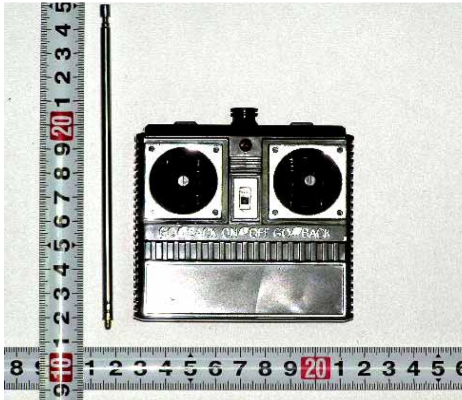
EUT - Front View
