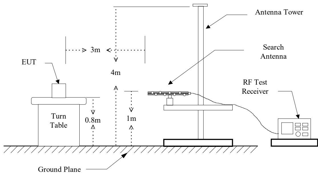
Figure 1(b) : Frequencies measured below 1 GHz configuration
