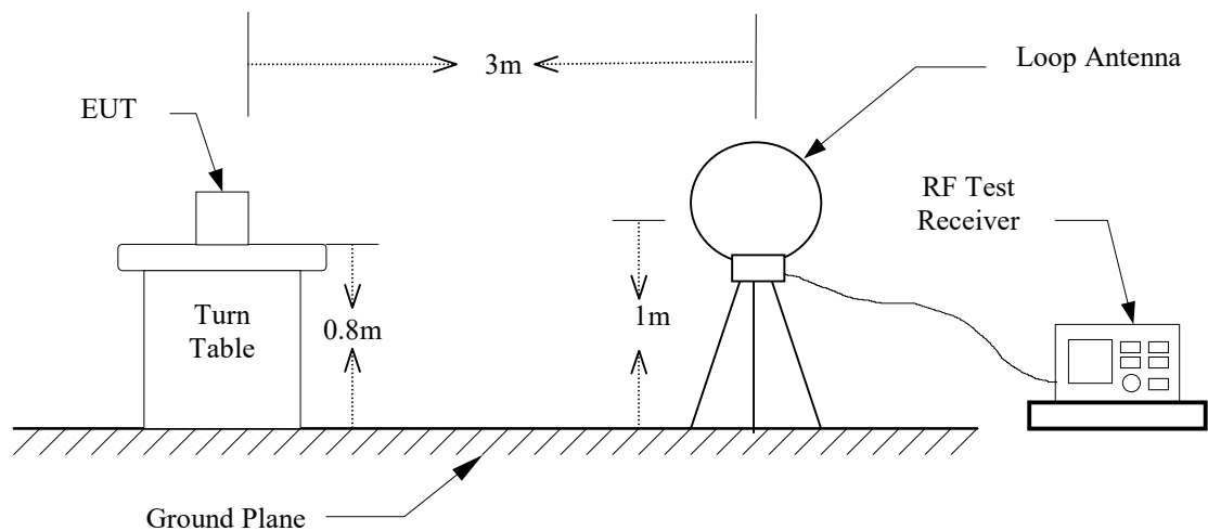
Figure 1(b) : Frequencies measured below 1 GHz configuration
