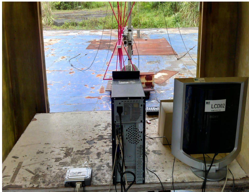
< RE Rear View >
