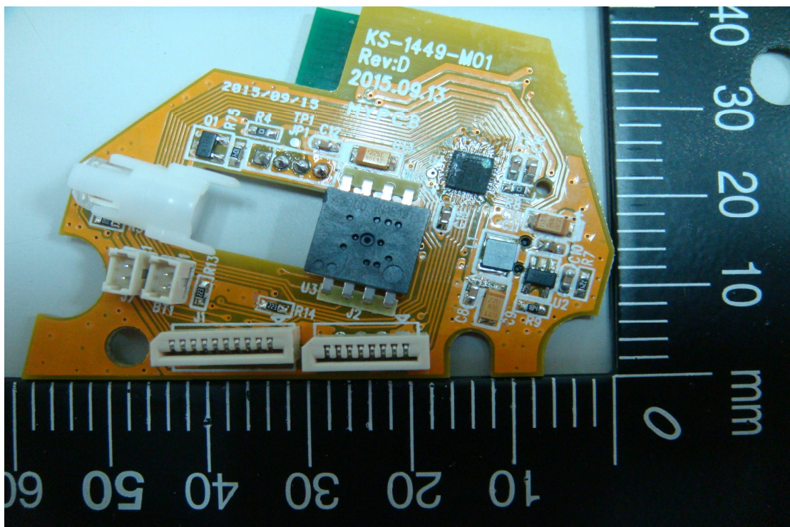
< PCB3-F >
