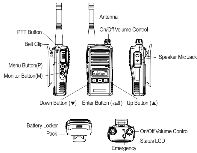
figure 3-1) Appearance of EZ1 Series Radio
