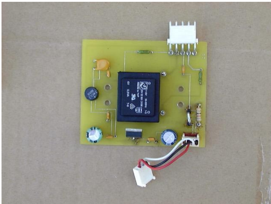
Figure 6 AC Power Supply Side 1
