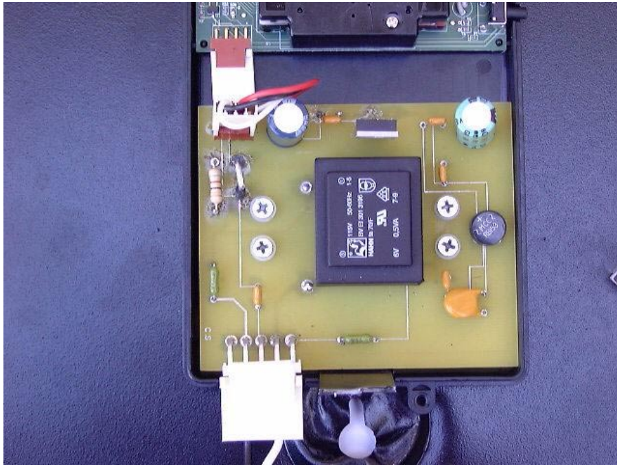
Figure 3 AC Power Supply in Case
