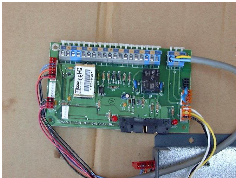
Figure 10 Communication Converter Card Side 2
