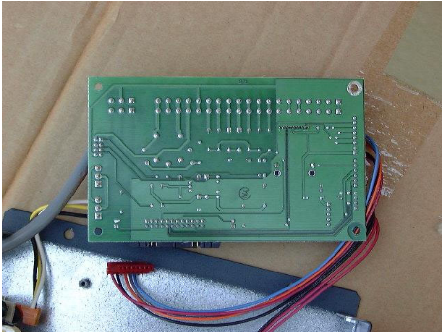
Figure 9 Communication Converter Card Side 1
