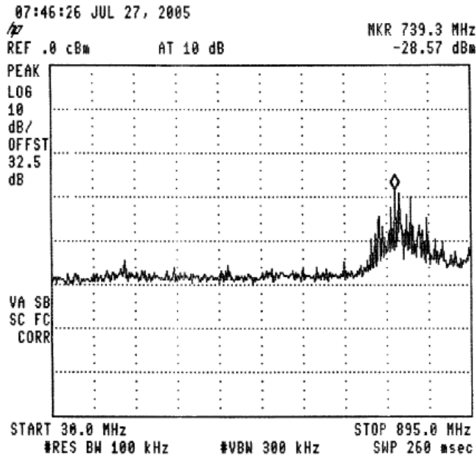
Figure 34.— 914.81 MHz
