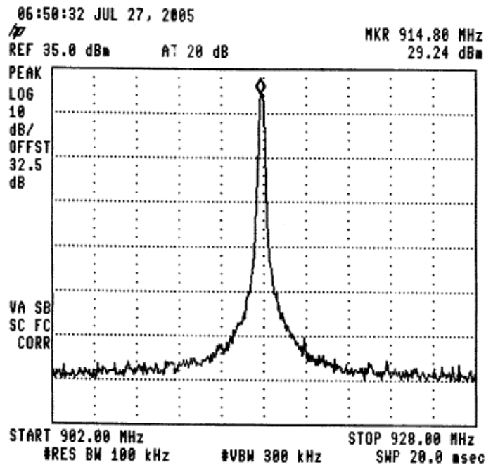
Figure 30.— 914.81 MHz
