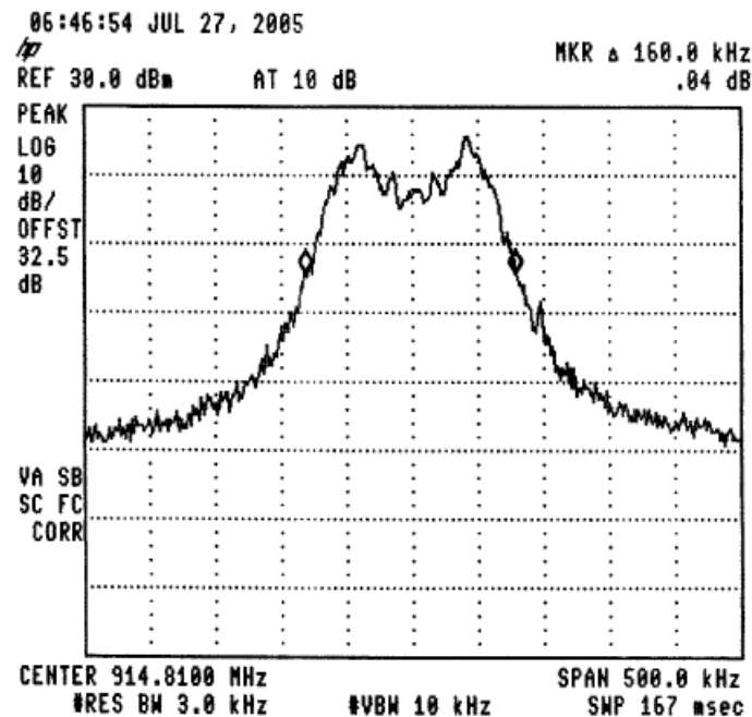
Figure 62 — 914.81 MHz
