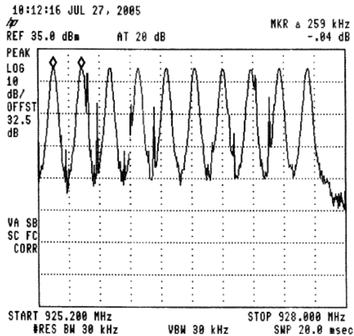
Figure 19.— 925.2-928.0 MHz
