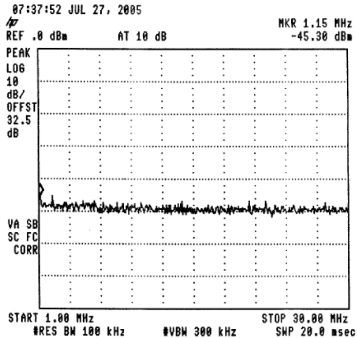
Figure 33.— 914.81 MHz
