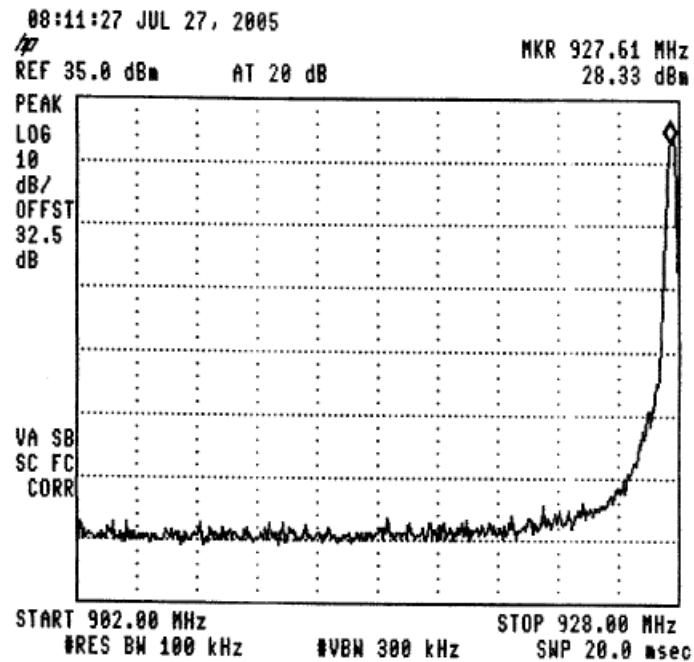
Figure 50.— 927.61 MHz
