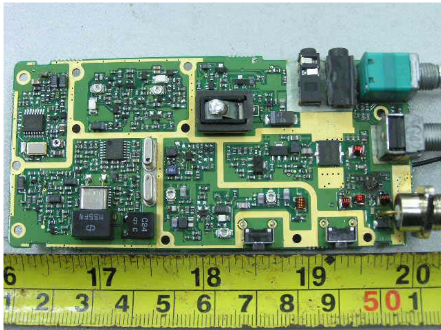
EUT – Main PCB Front View
