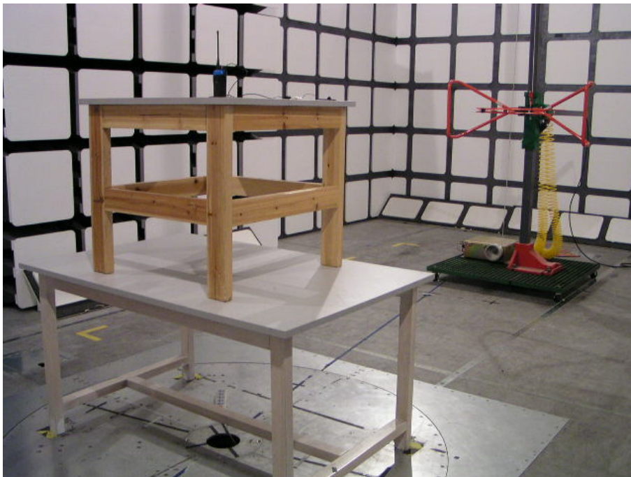
Radiated Emission - Rear View (30-1000 MHz)
