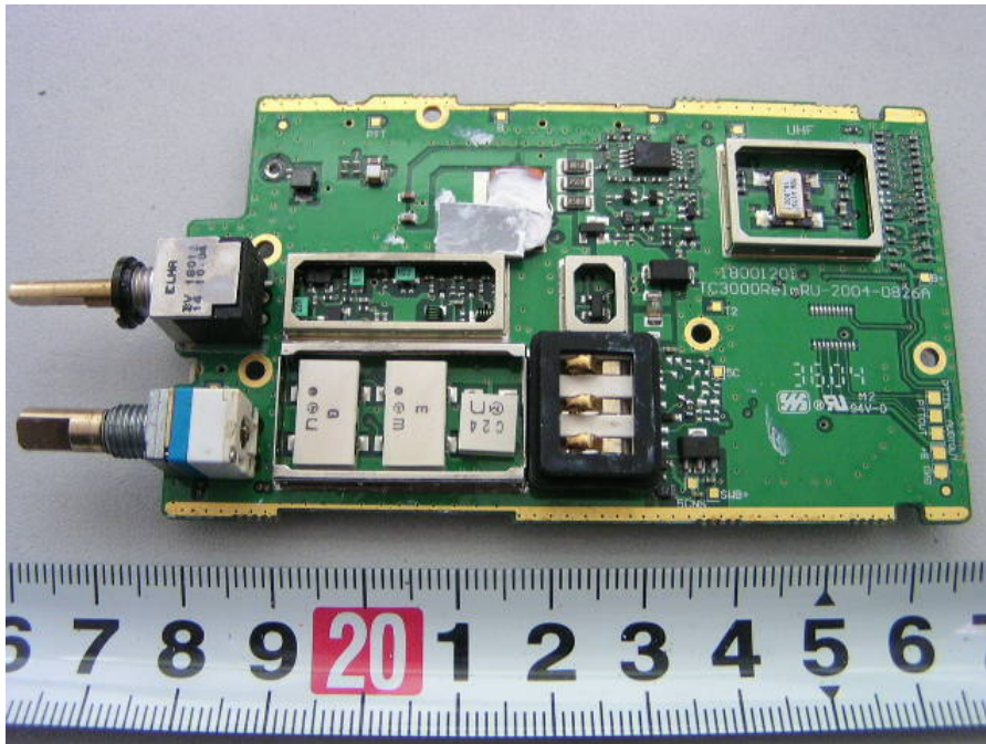
Board – Bottom Shield Cover Removed View
