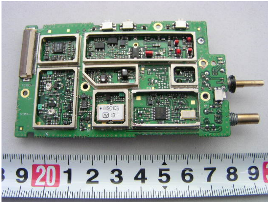
Board – Top Shield Cover Removed View
