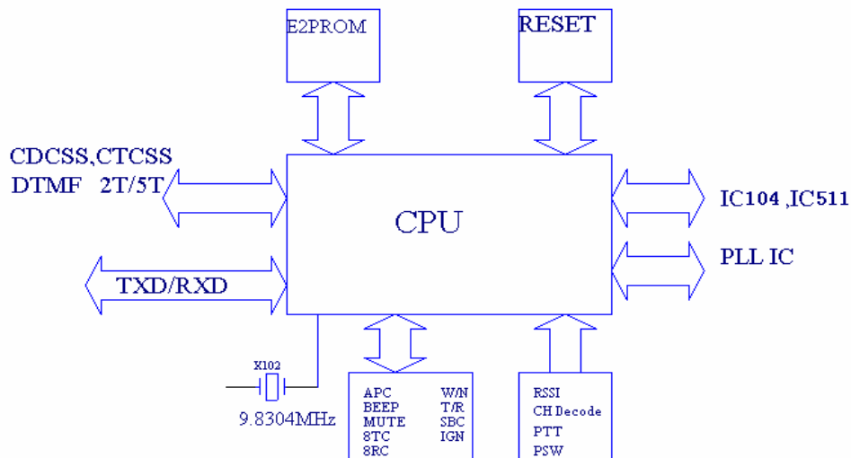
Fig4 Control Circuit
