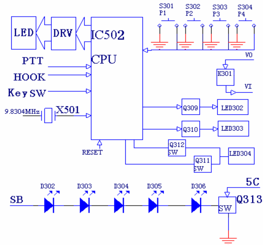
Fig6. Display Circuit
