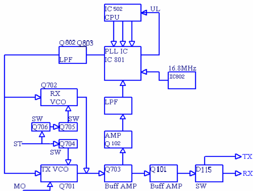
Fig3 PLL Circuit
