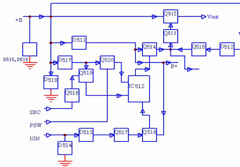
Fig 5 Power Switch Circuit
