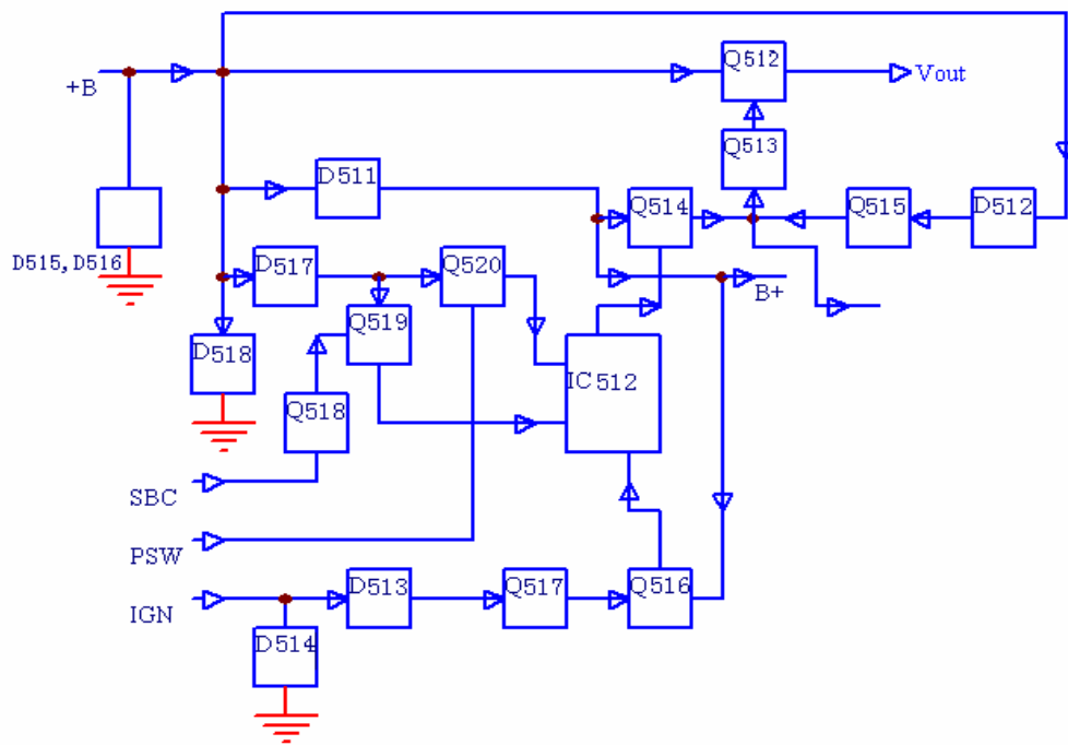
Power Switch Circuit Block Diagram
