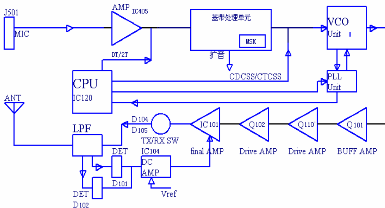
Transmitting Part Block Diagram
