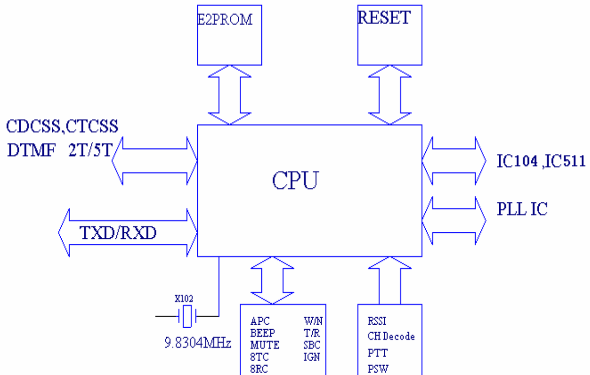
Controlling Circuit Block Diagram
