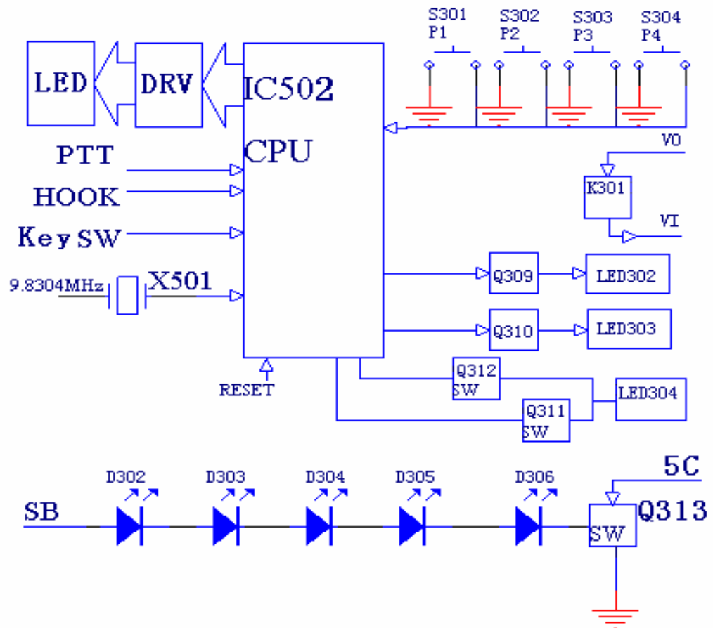
Display Circuit Block Diagram
