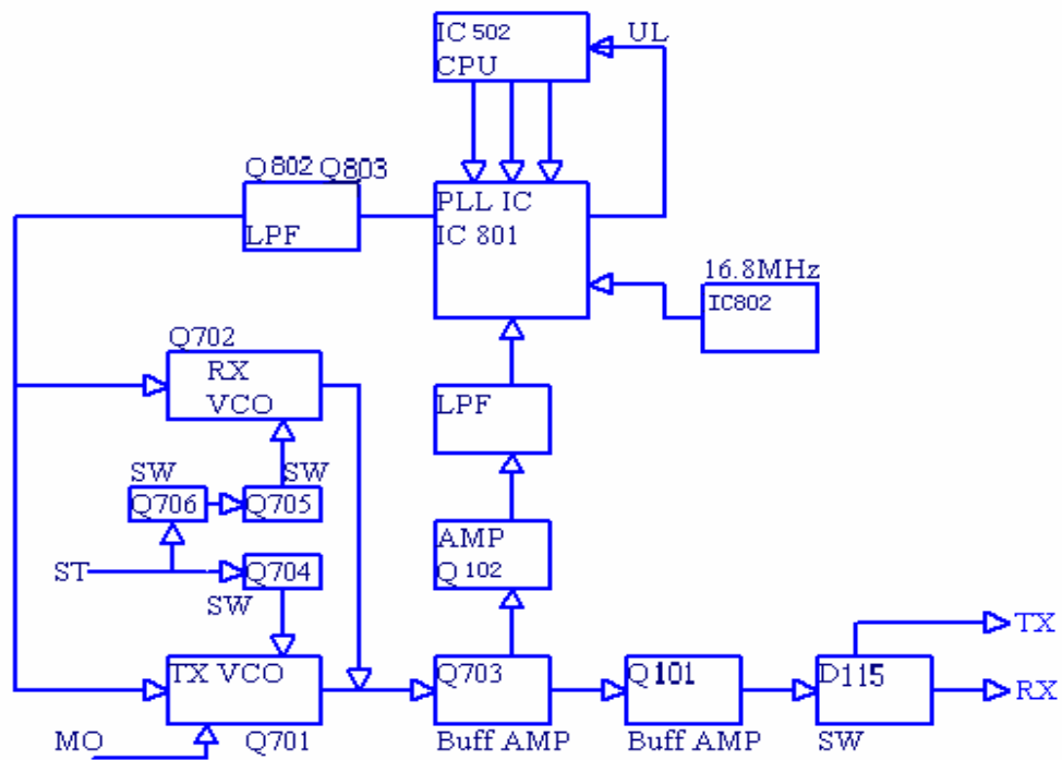
PLL Circuit Block Diagram
