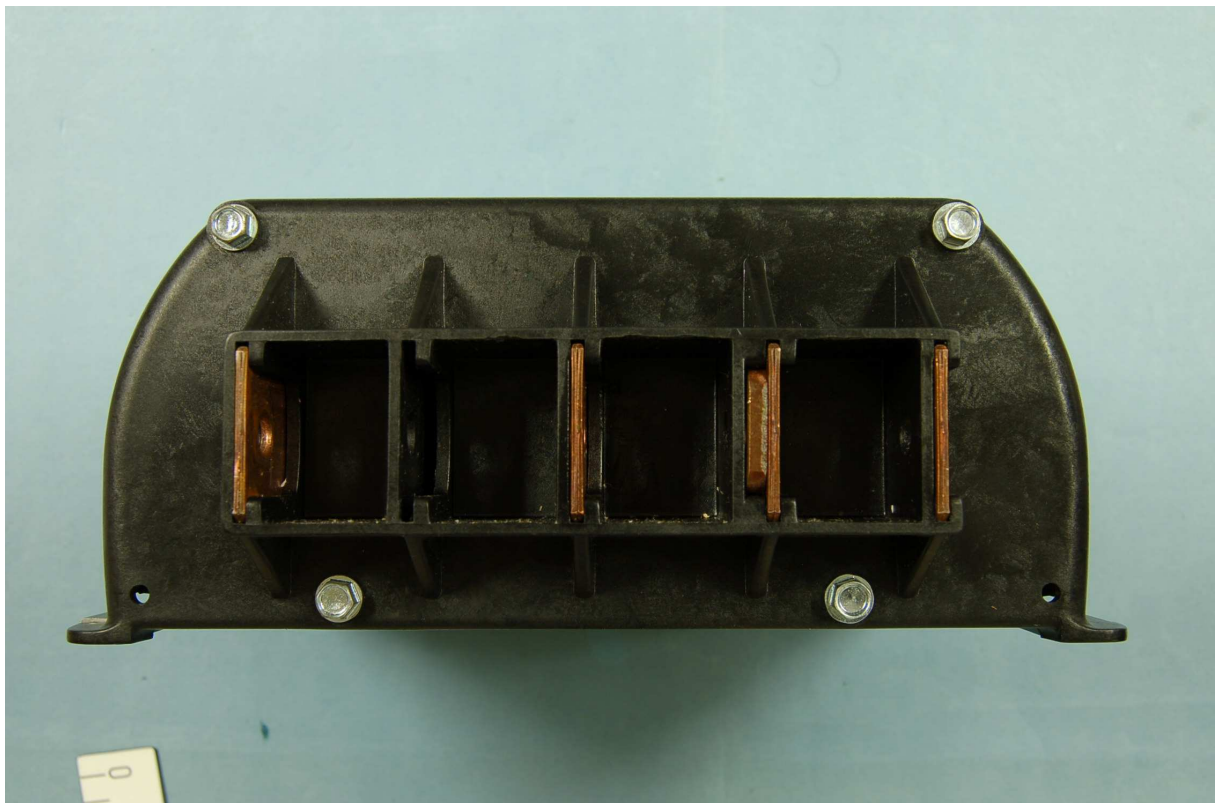
ECU-01 – View of the connector side
