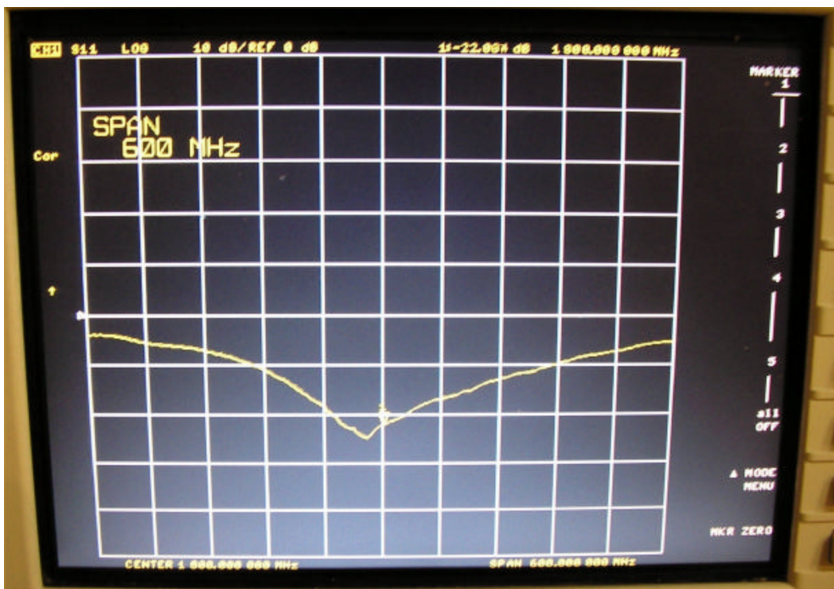
1800MHz dipole validation return loss data 8/20/2004
