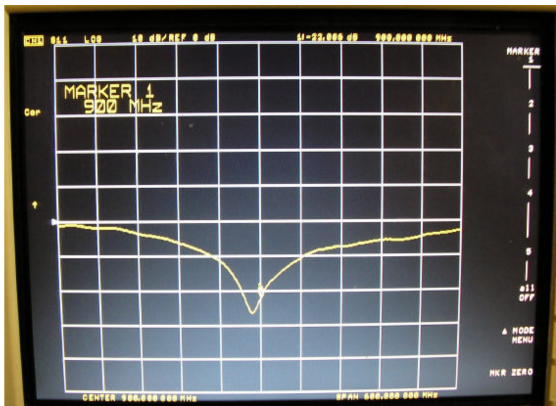
900 MHz validation return loss data 8/20/2004
