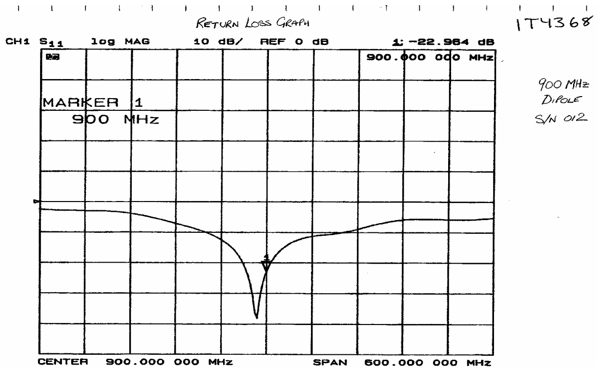
900MHz Dipole MFR return loss Data
