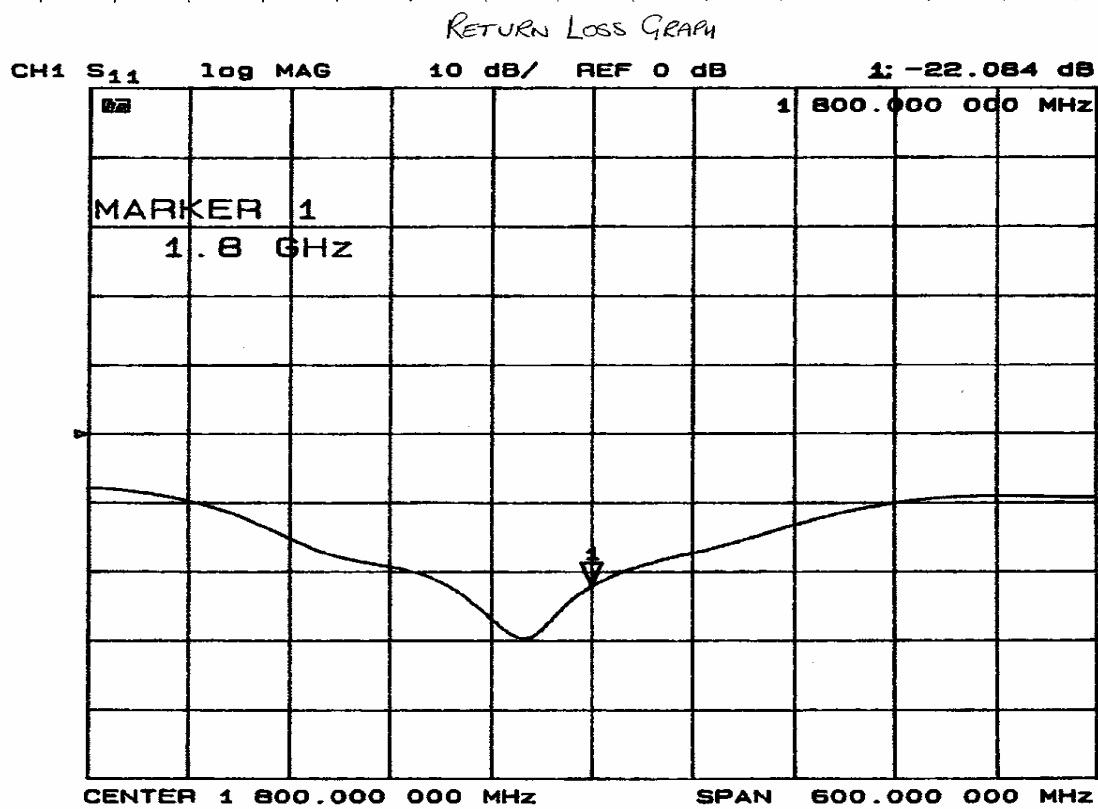
1800MHz Dipole MFR return loss Data
