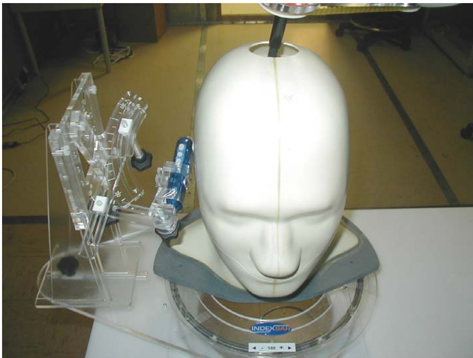
Figure S2. Setup Configuration of Right Ear Cheek and Tilt ( 850/1900 Head SAR)
