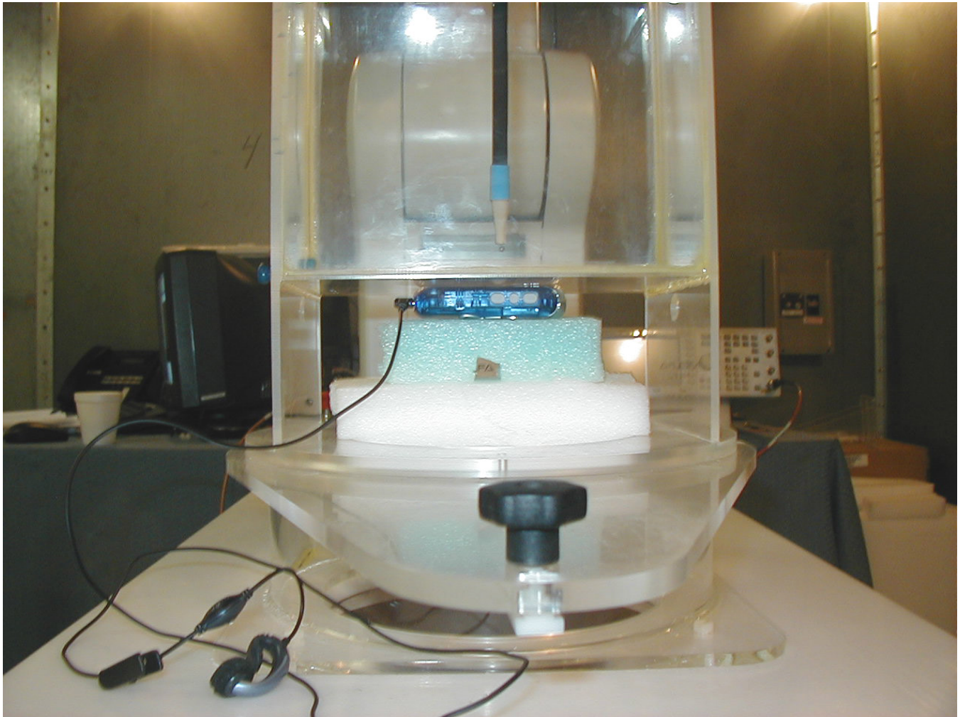
Figure S2. Setup Configuration of Body SAR
