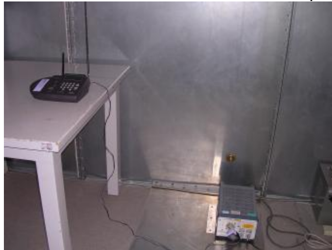
Measurement of Conducted Emission Test Set Up
