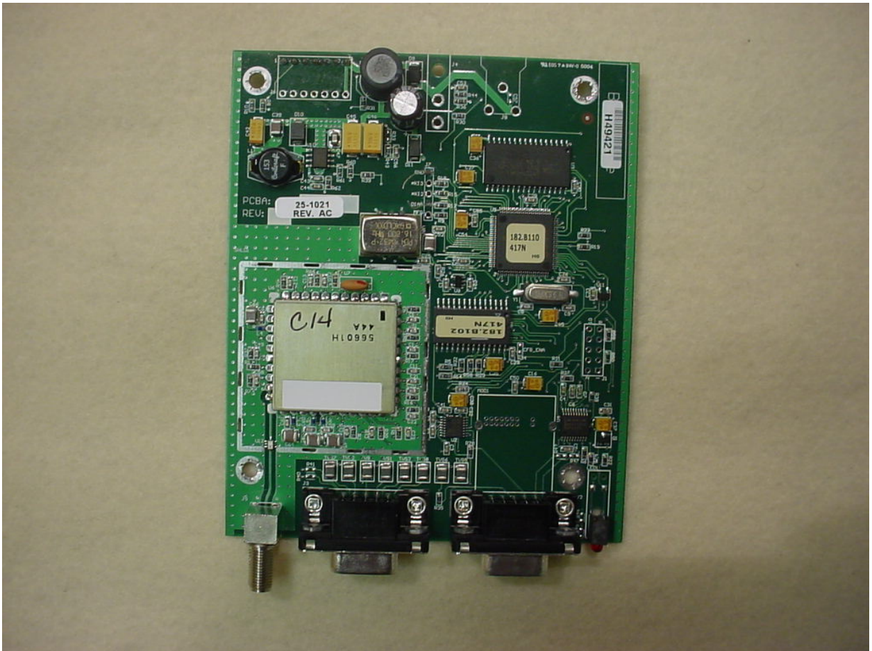
Figure 1: Internal – Integrated Wangate Radio Board – Front
