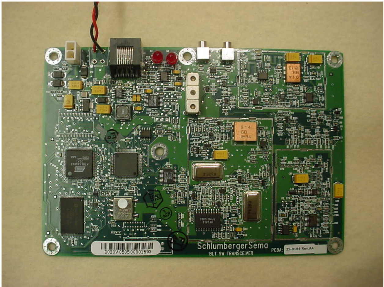
Figure 3: Internal – BLT Radio Board – Front
