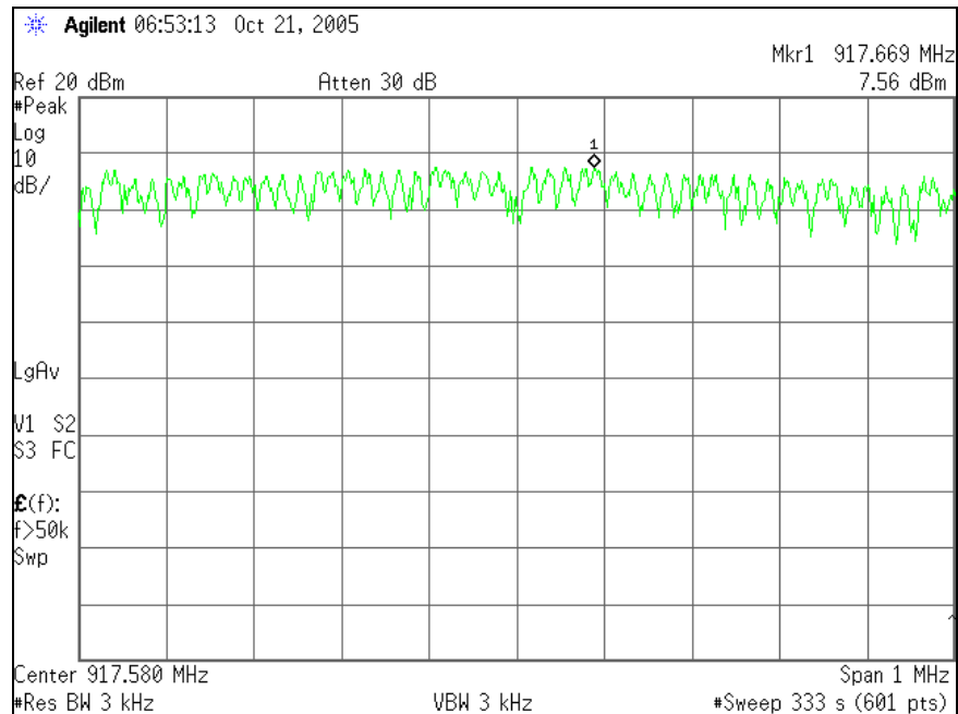
Figure 7.7.2-1: Peak Power Spectral Density
