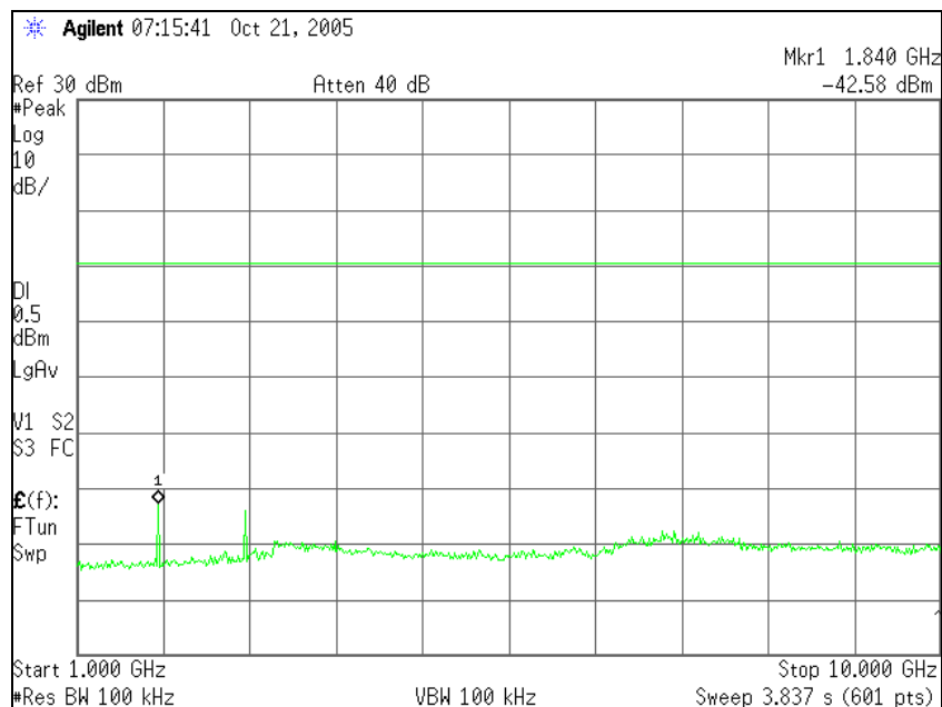
Figure 7.6.2.2-2: RF Conducted Spurious Emission 1 GHz – 10 GHz
