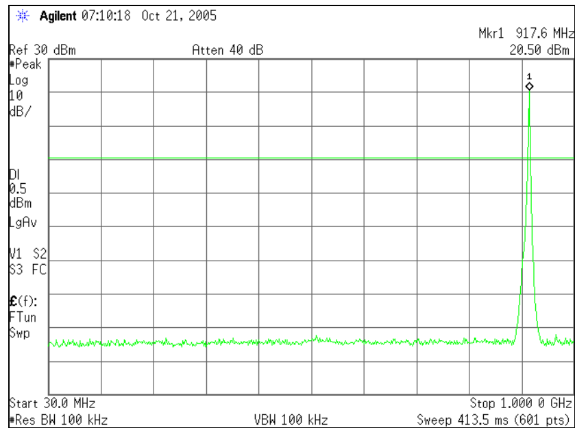
Figure 7.6.2.2-1: RF Conducted Spurious Emission 30 MHz – 1 GHz
