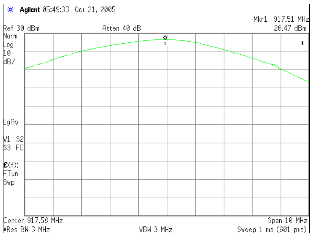
Figure 7.5.2-1: Output power
