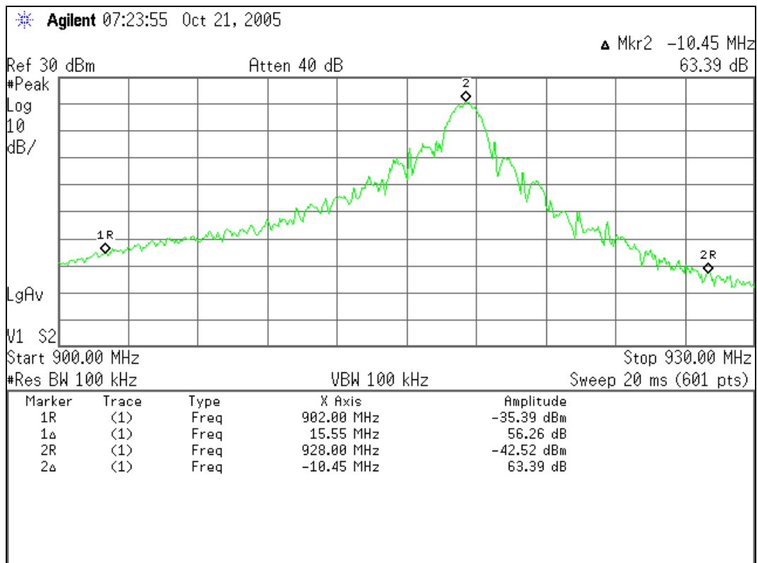
Figure 7.6.1.2-1: Band-edge
