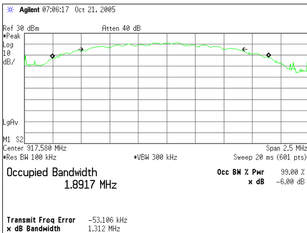
Figure 7.4.2-1: 6dB Bandwidth Plot
