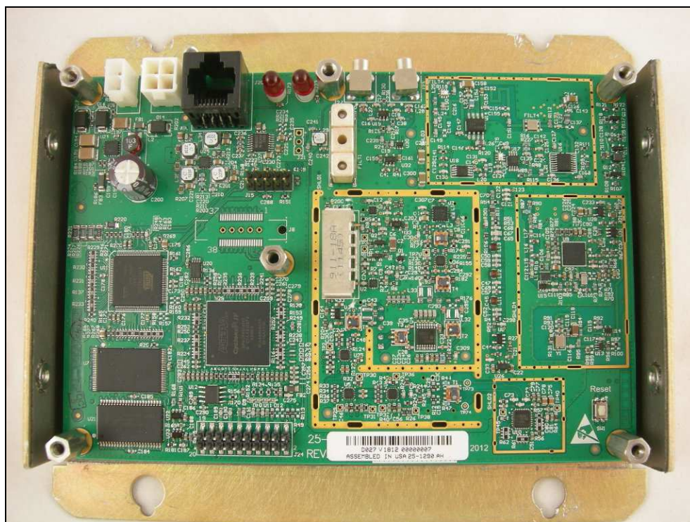
Figure 1: Internal Photo – PCB Top
