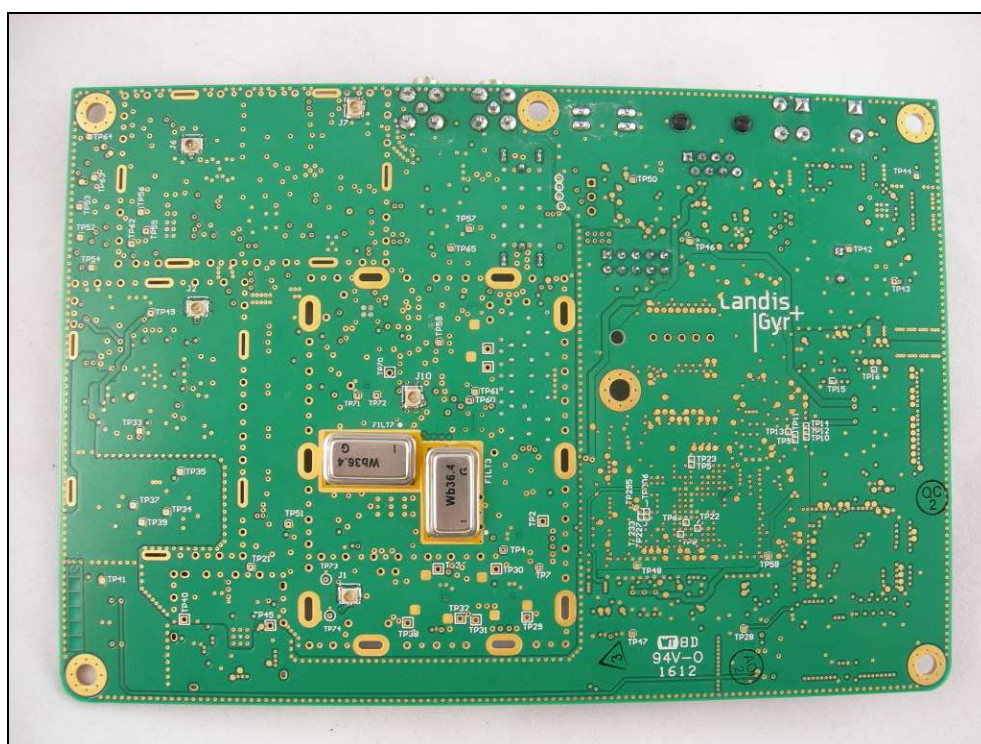
Figure 2: Internal Photo – PCB Bottom
