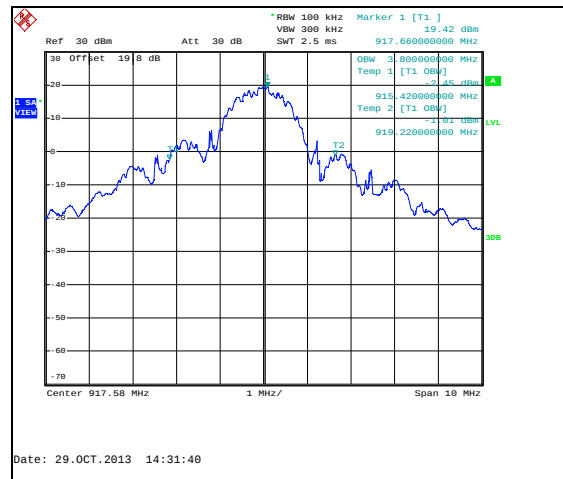
Figure 7.3.2-2: 99% Bandwidth Plot – Port A
