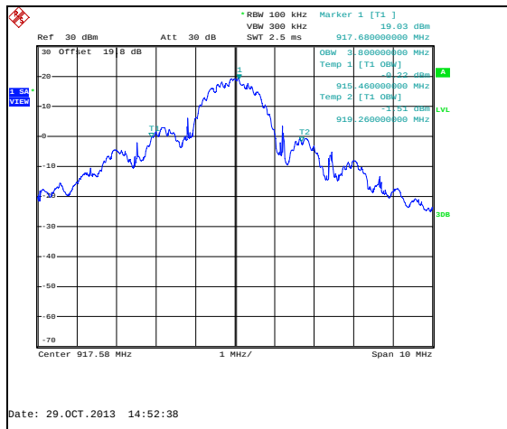
Figure 7.3.2-4: 99% Bandwidth Plot – Port B
