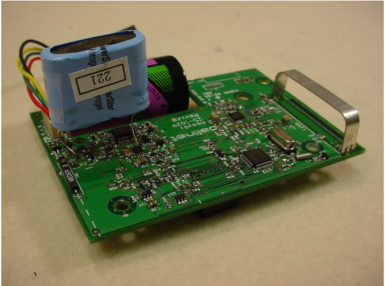
Figure 3: Internal – Top View - PCB
