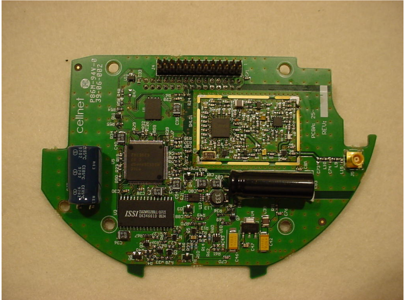
Figure 2: Internal - PCB Front No Shield
