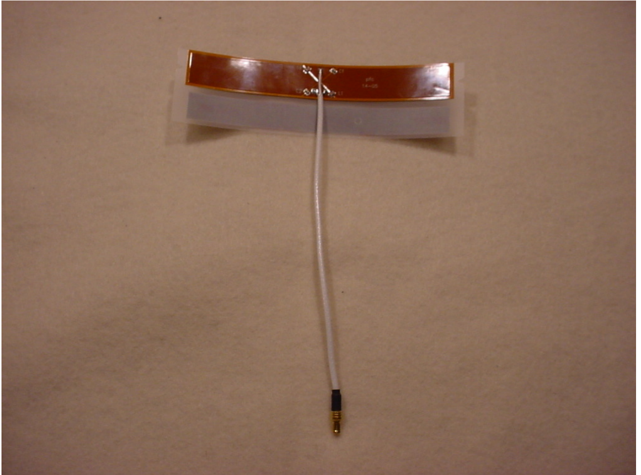
Figure 5: Antenna Back
