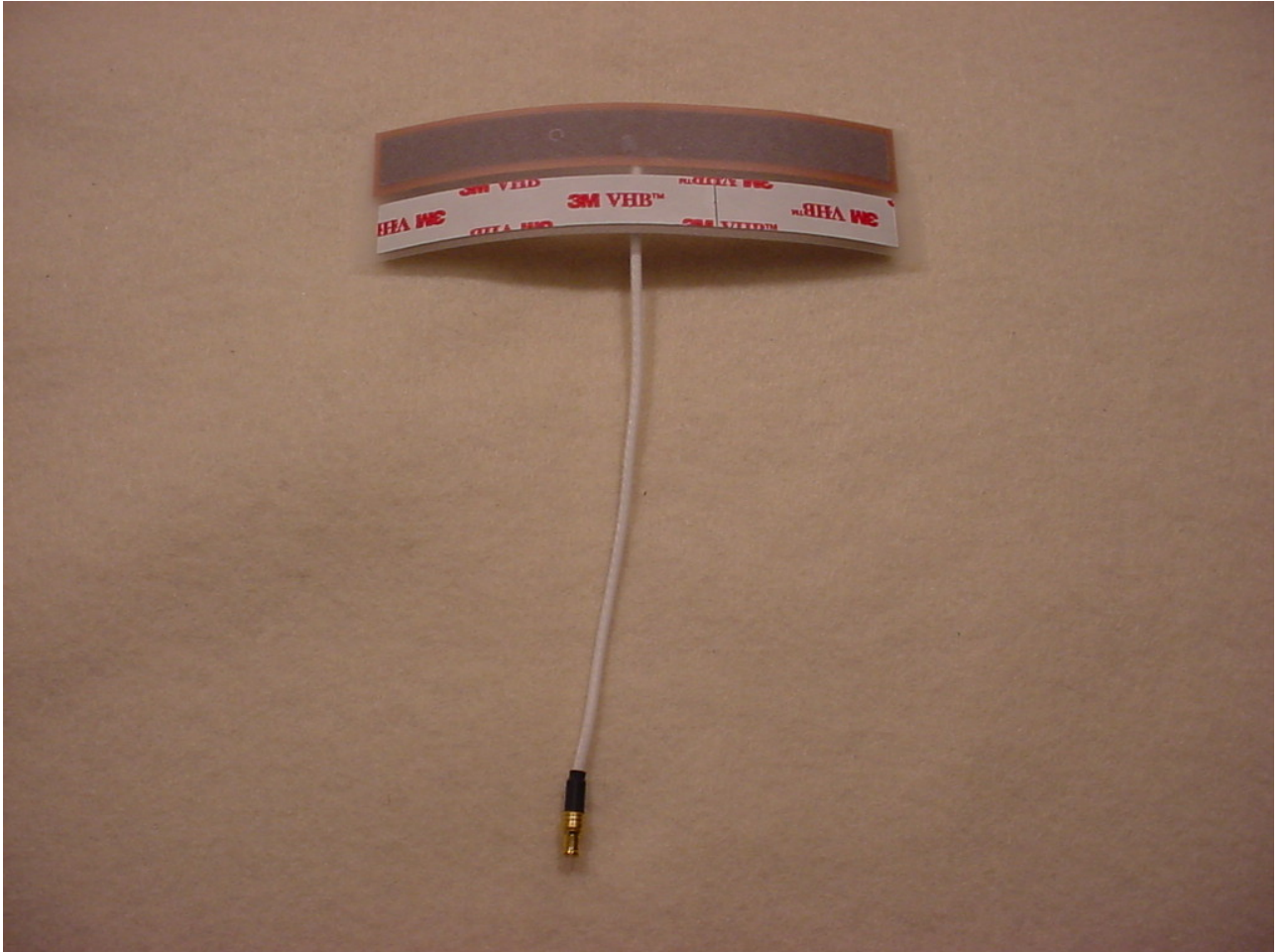
Figure 4: Antenna Front
