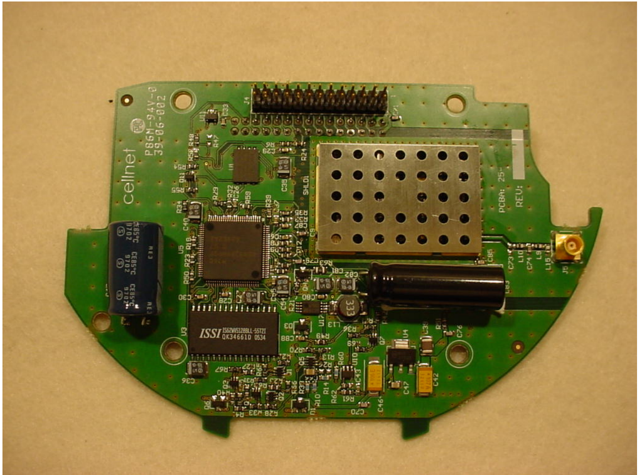
Figure 1: Internal - PCB Front Shielded
