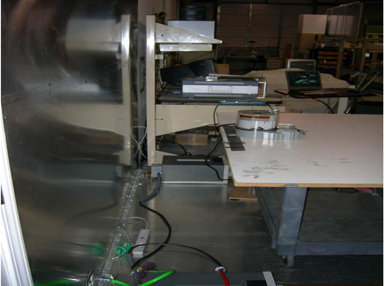
Figure 6: Test Setup - Conducted Emissions
