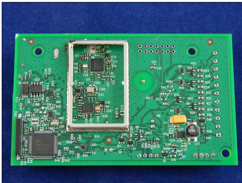
Figure 1: Internal Photo – Shield Removed
