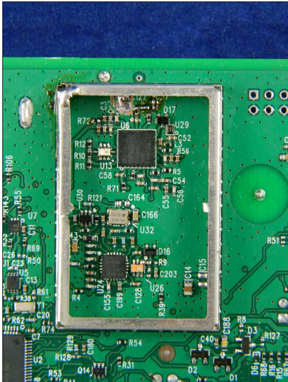
Figure 2: Internal Photo – Shield Removed
