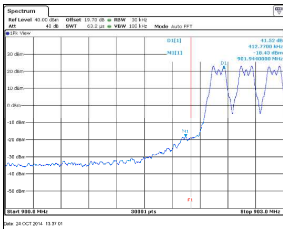
Figure 7.5.1.2-9: Lower Band-edge – Mode 1
