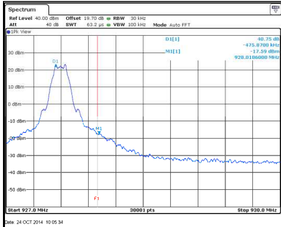
Figure 7.5.1.2-8: Upper Band-edge – Mode 4
