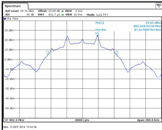
Figure 7.4.4.2-24: 99% BW Low Channel - 38.4kbps
