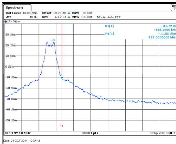
Figure 7.5.1.2-5: Upper Band-edge – Mode 1
