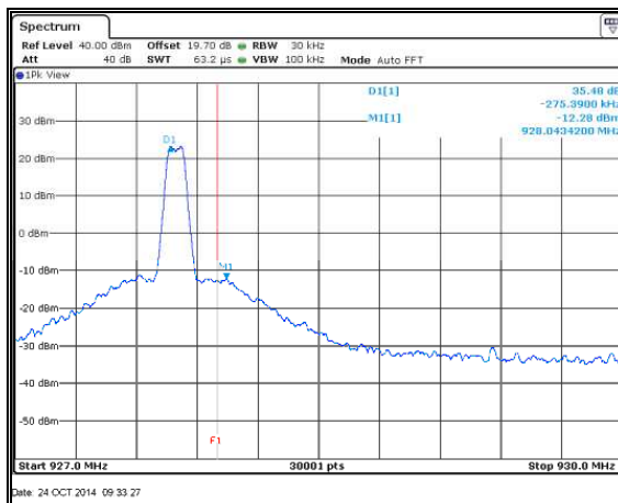
Figure 7.5.1.2-7: Upper Band-edge – Mode 3
