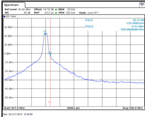
Figure 7.5.1.2-6: Upper Band-edge – Mode 2
