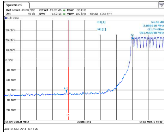
Figure 7.5.1.2-10: Lower Band-edge – Mode 2
